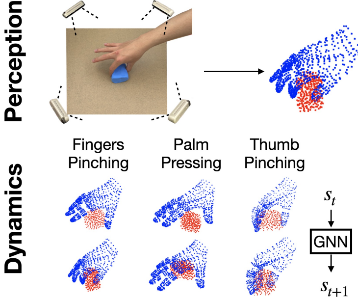
Fig. 1: Overall framework. The perception module captures a clear and consistent particle-based representation of the scene using four RGBD cameras. Leveraging this representation, our method learns a dynamics model from diverse hand-object interactions across multiple manipulation skills, including Fingers Pinching, Palm Pressing, and Thumb Pinching. During cross-embodiment planning, the learned dynamics model is employed to manipulate deformable objects toward desired target states.
