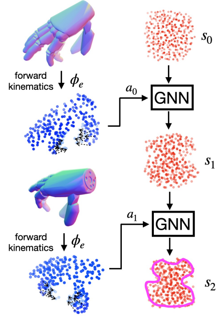
Fig. 1: Overall framework. The perception module captures a clear and consistent particle-based representation of the scene using four RGBD cameras. Leveraging this representation, our method learns a dynamics model from diverse hand-object interactions across multiple manipulation skills, including Fingers Pinching, Palm Pressing, and Thumb Pinching. During cross-embodiment planning, the learned dynamics model is employed to manipulate deformable objects toward desired target states.
